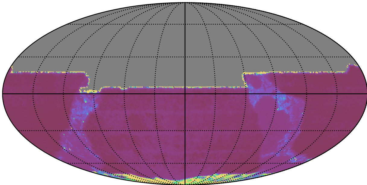
weather_cloudso12v3.4_10yrs All sky y band: Median Inter-Night Gap
