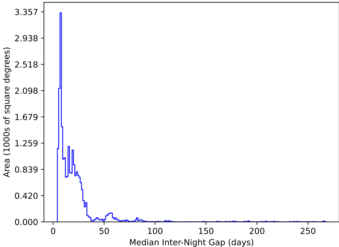
weather_cloudso12v3.4_10yrs All sky y band: Median Inter-Night Gap
