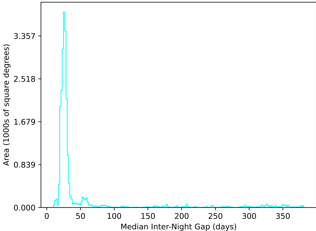
weather_cloudso12v3.4_10yrs All sky u band: Median Inter-Night Gap
