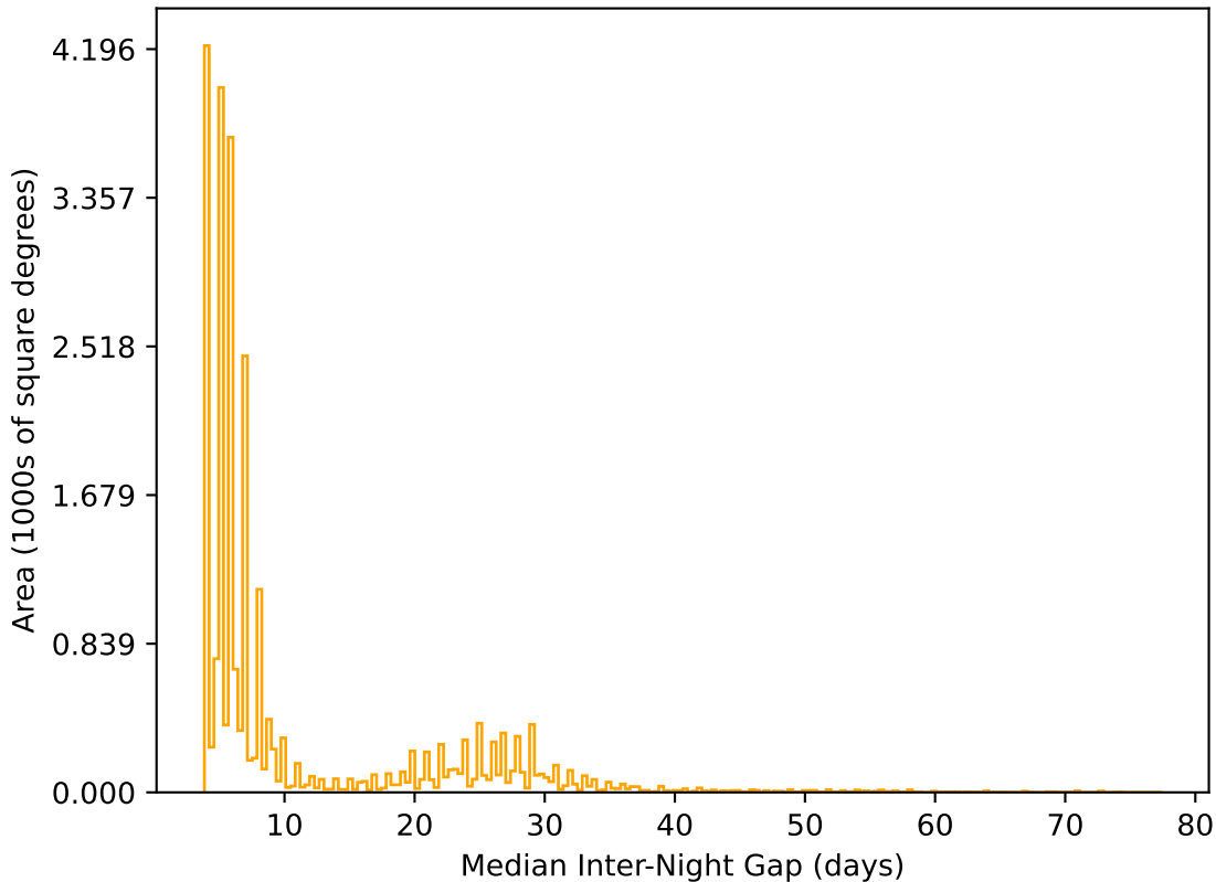
weather_cloudso12v3.4_10yrs All sky r band: Median Inter-Night Gap
