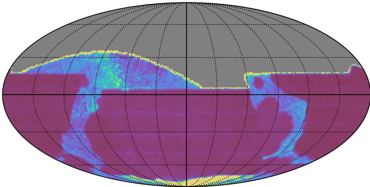
weather_cloudso12v3.4_10yrs All sky i band: Median Inter-Night Gap
