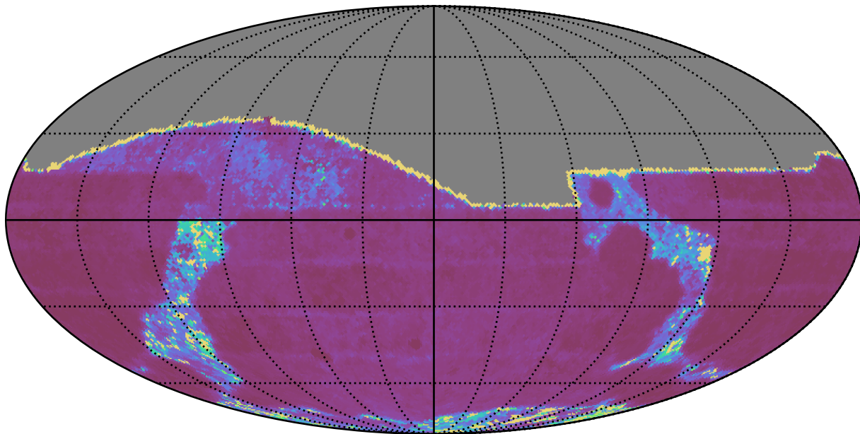
weather_cloudso12v3.4_10yrs All sky g band: Median Inter-Night Gap
