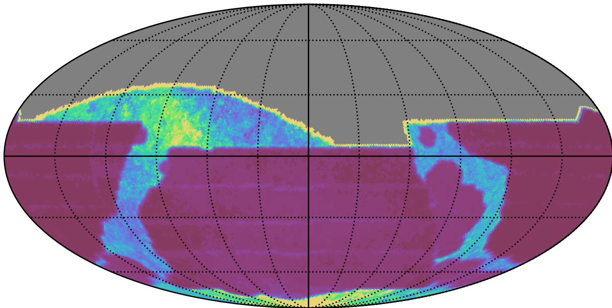
weather_cloudso12v3.4_10yrs All sky all bands: Median Inter-Night Gap
