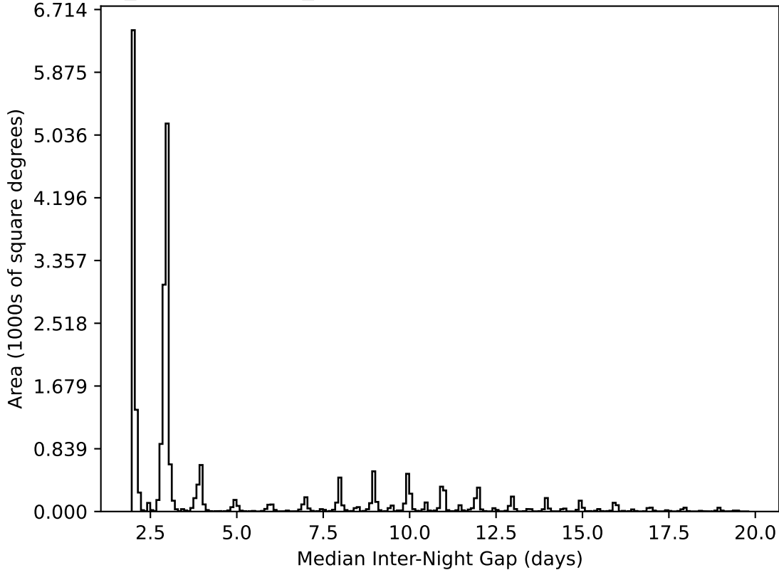
weather_cloudso12v3.4_10yrs All sky all bands: Median Inter-Night Gap
