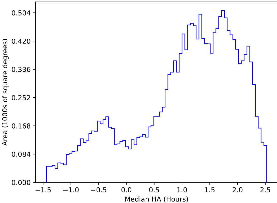
weather_cloudso12v3.4_10yrs WFD z band: Median HA
