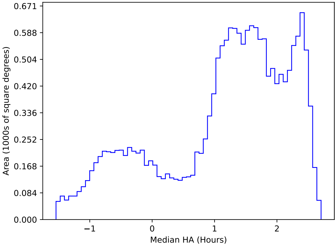
weather_cloudso12v3.4_10yrs WFD y band: Median HA
