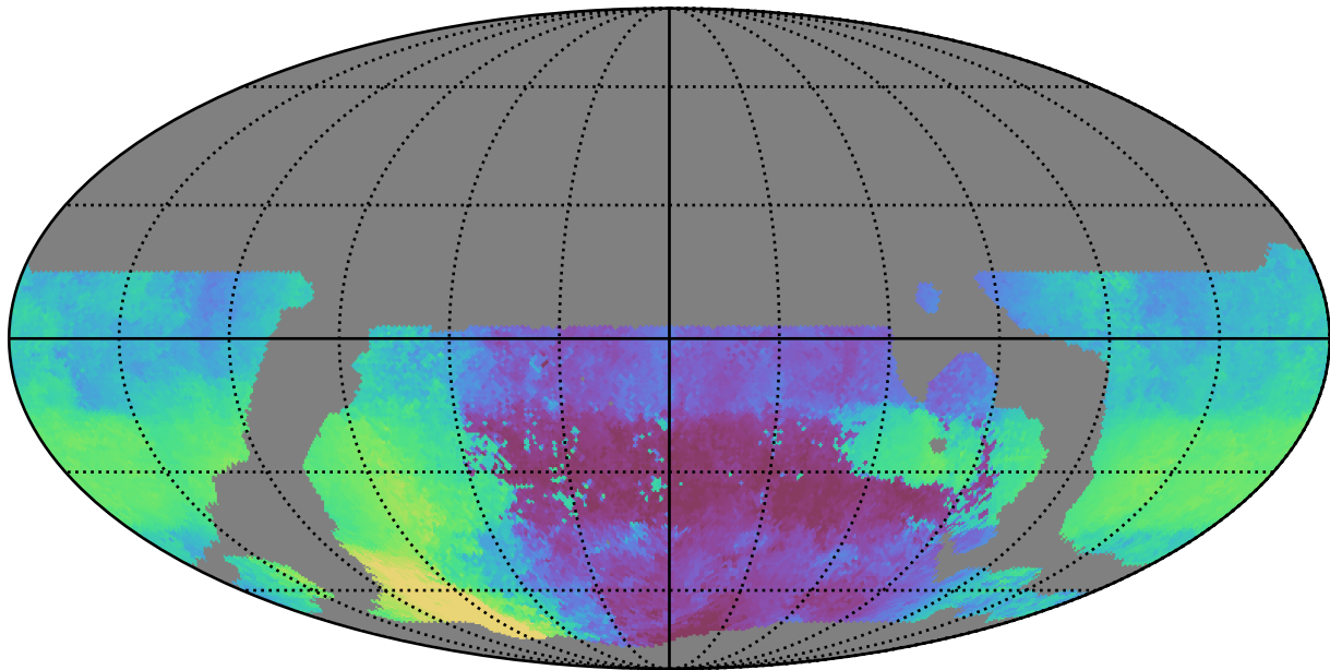
weather_cloudso12v3.4_10yrs WFD u band: Median HA
