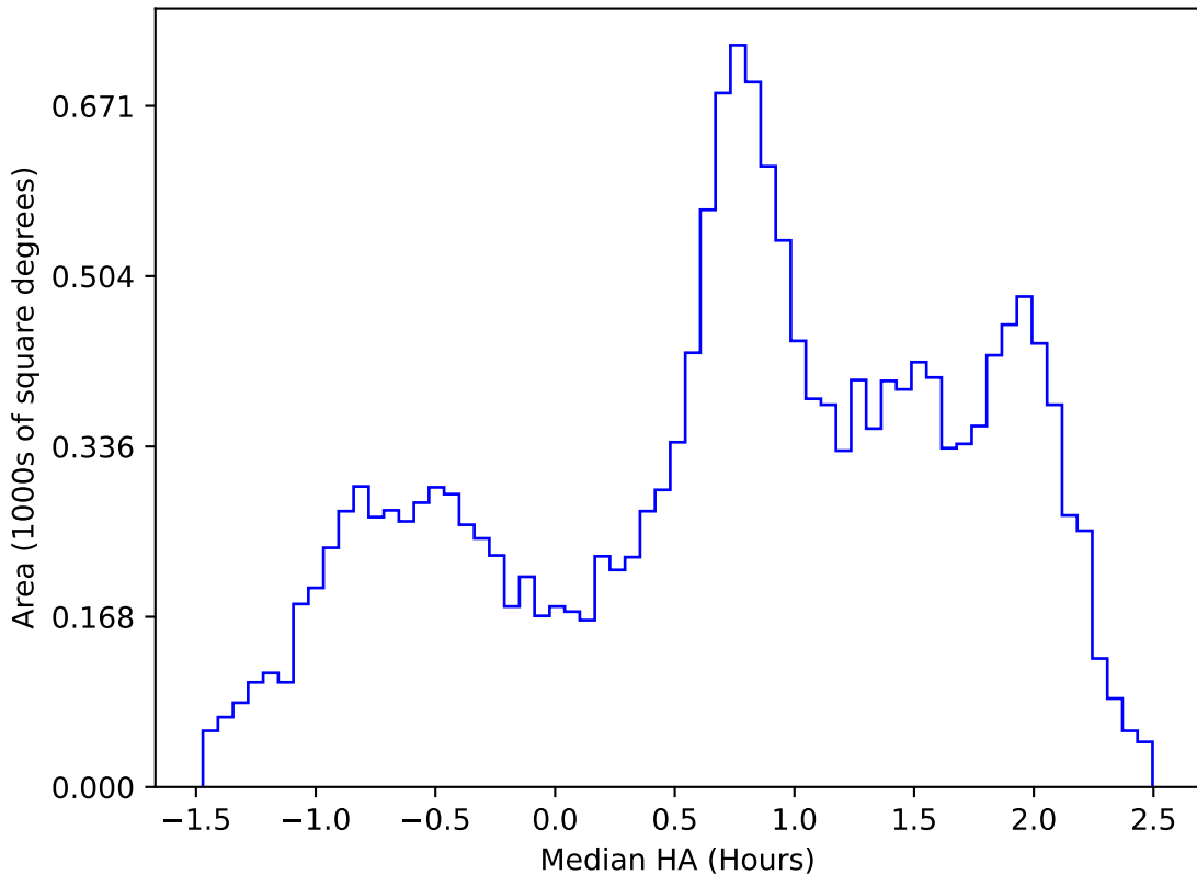
weather_cloudso12v3.4_10yrs WFD r band: Median HA
