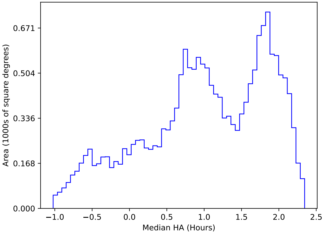
weather_cloudso12v3.4_10yrs WFD i band: Median HA
