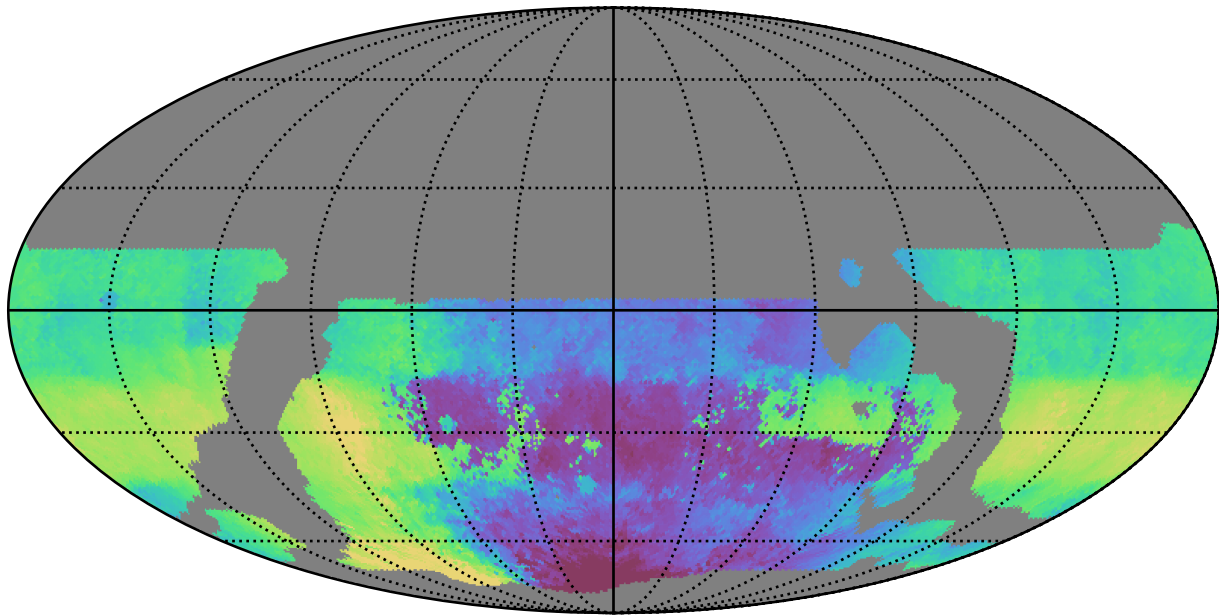
weather_cloudso12v3.4_10yrs WFD g band: Median HA
