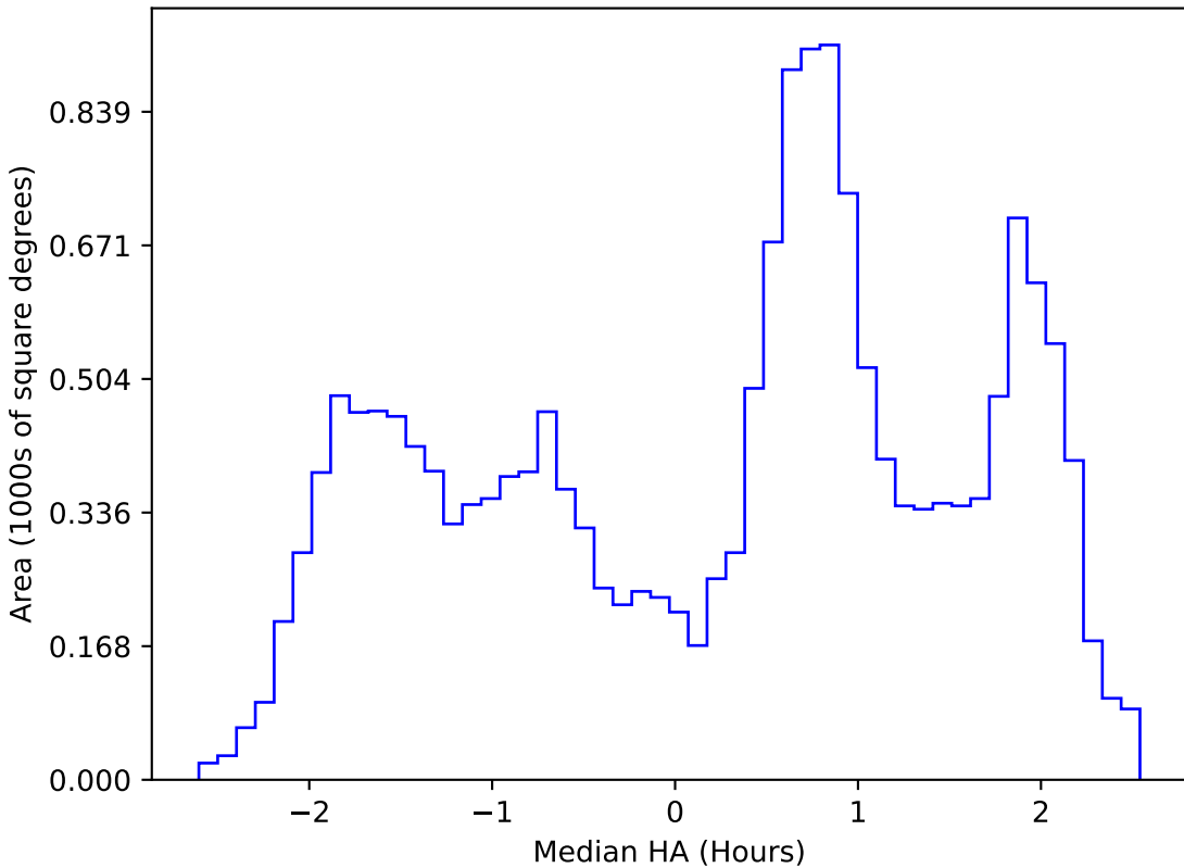
weather_cloudso12v3.4_10yrs WFD g band: Median HA
