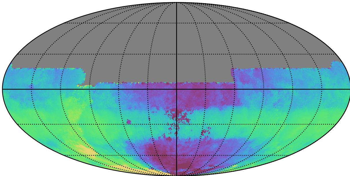
weather_cloudso12v3.4_10yrs All sky y band: Median HA
