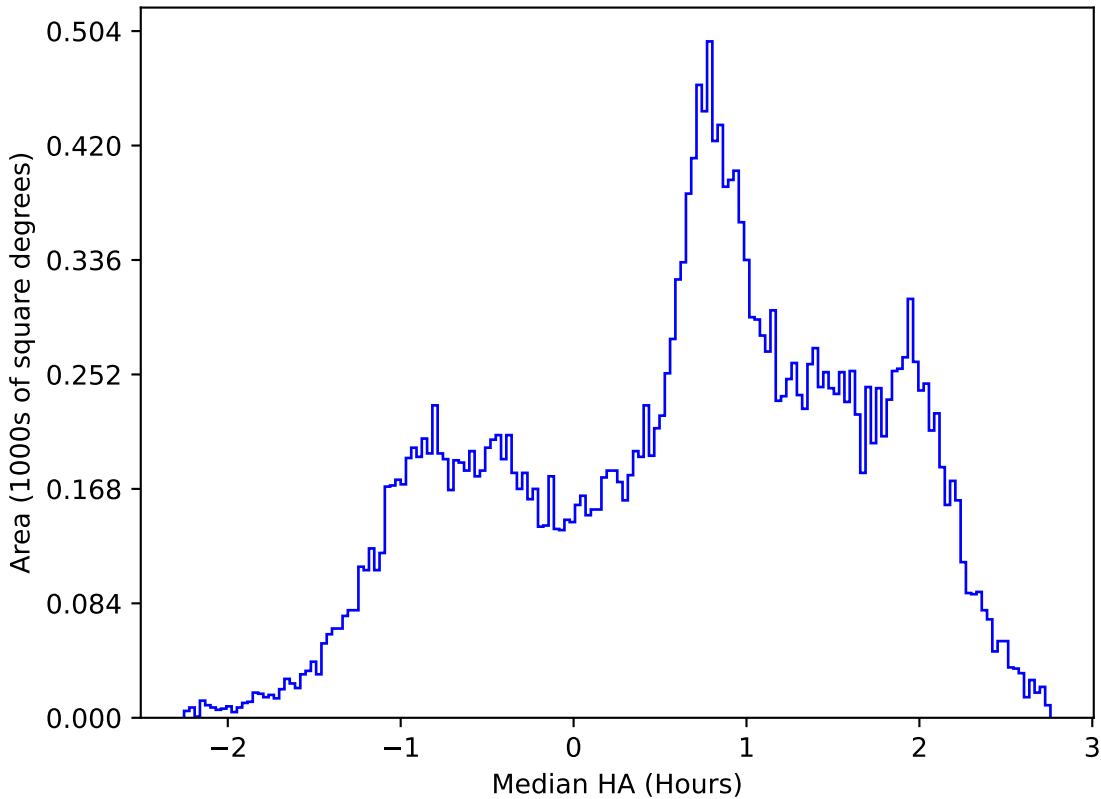
weather_cloudso12v3.4_10yrs All sky r band: Median HA
