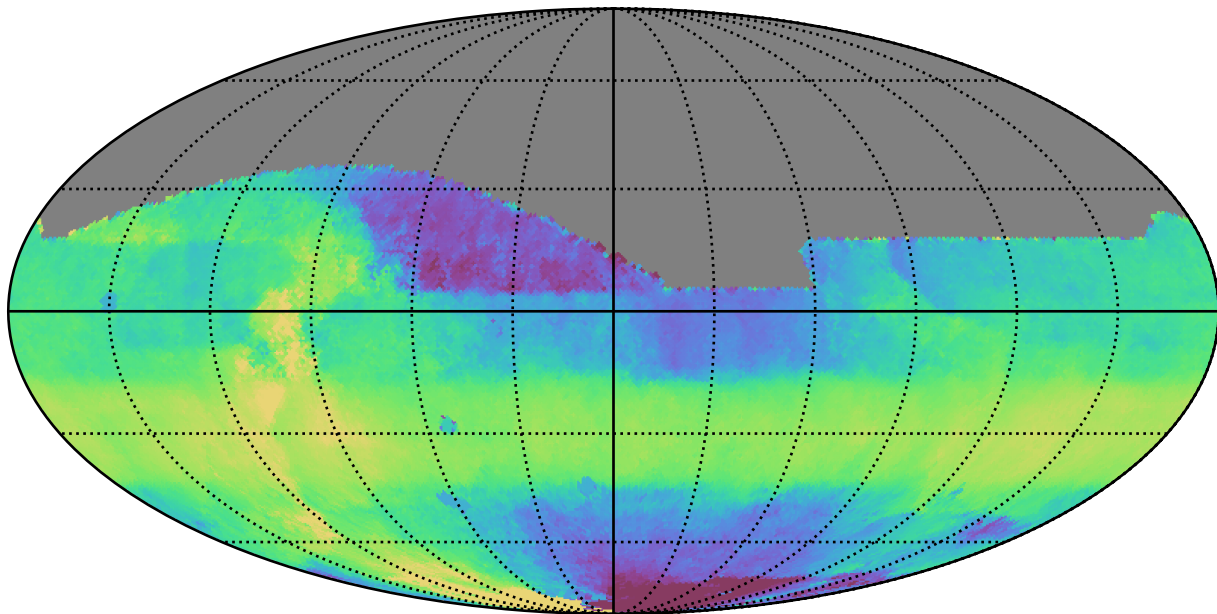
weather_cloudso12v3.4_10yrs All sky i band: Median HA
