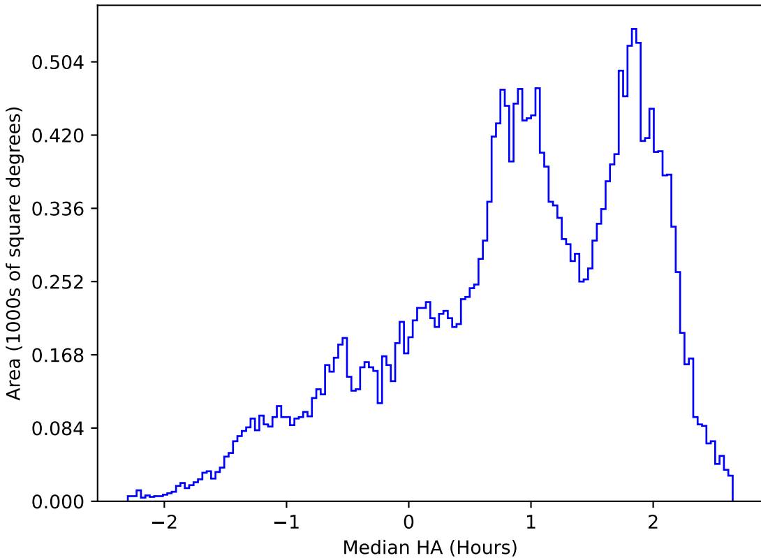
weather_cloudso12v3.4_10yrs All sky i band: Median HA
