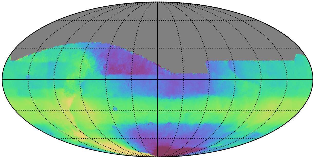
weather_cloudso12v3.4_10yrs All sky all bands: Median HA
