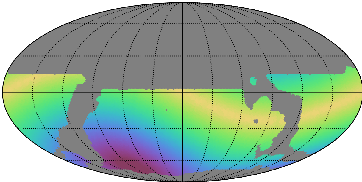
weather_cloudso12v3.4_10yrs WFD z band: Max solarElong
