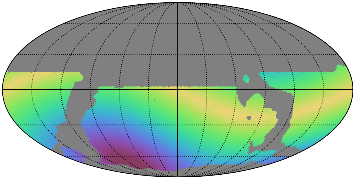
weather_cloudso12v3.4_10yrs WFD y band: Max solarElong
