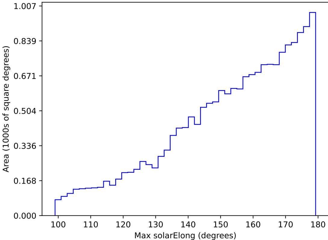
weather_cloudso12v3.4_10yrs WFD y band: Max solarElong
