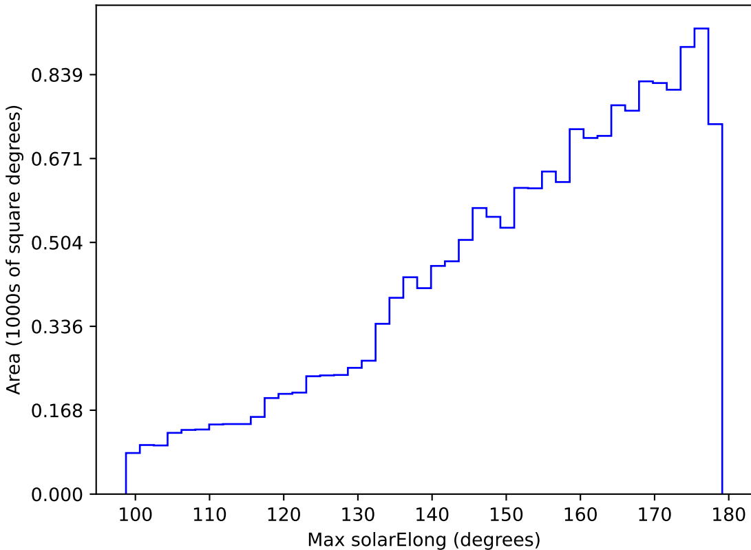
weather_cloudso12v3.4_10yrs WFD u band: Max solarElong
