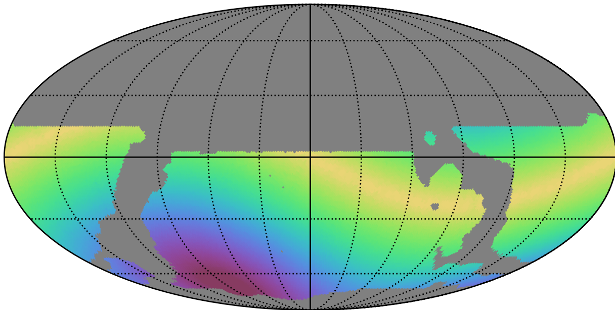
weather_cloudso12v3.4_10yrs WFD r band: Max solarElong
