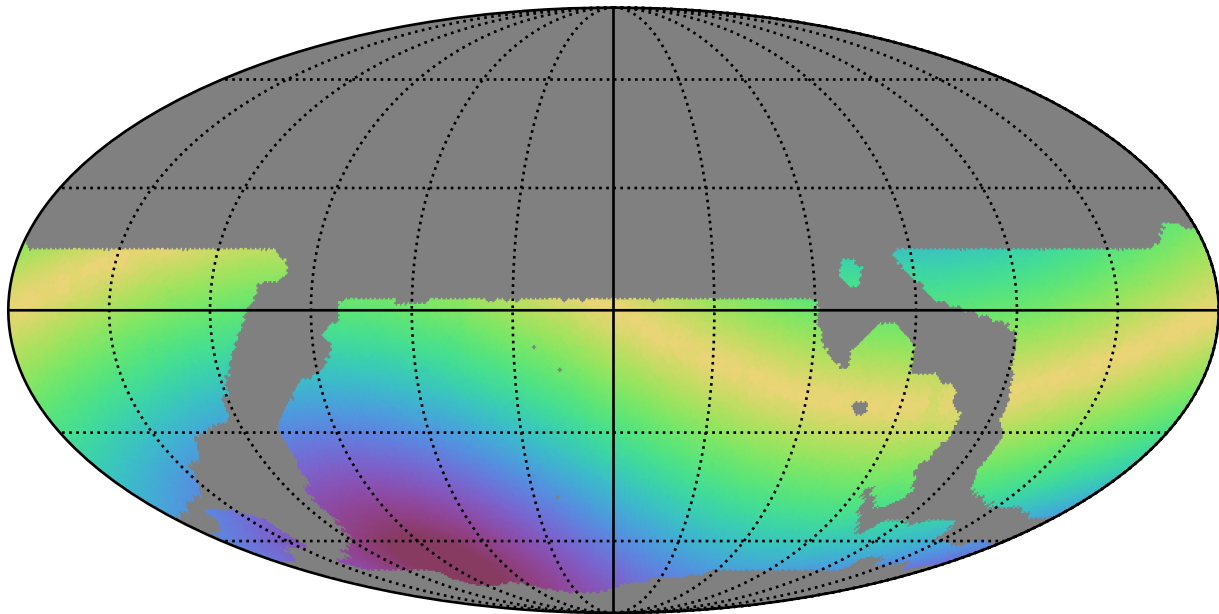
weather_cloudso12v3.4_10yrs WFD i band: Max solarElong
