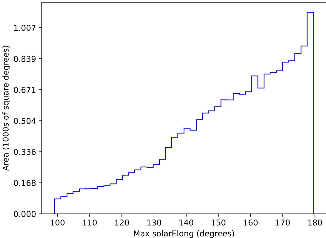
weather_cloudso12v3.4_10yrs WFD i band: Max solarElong
