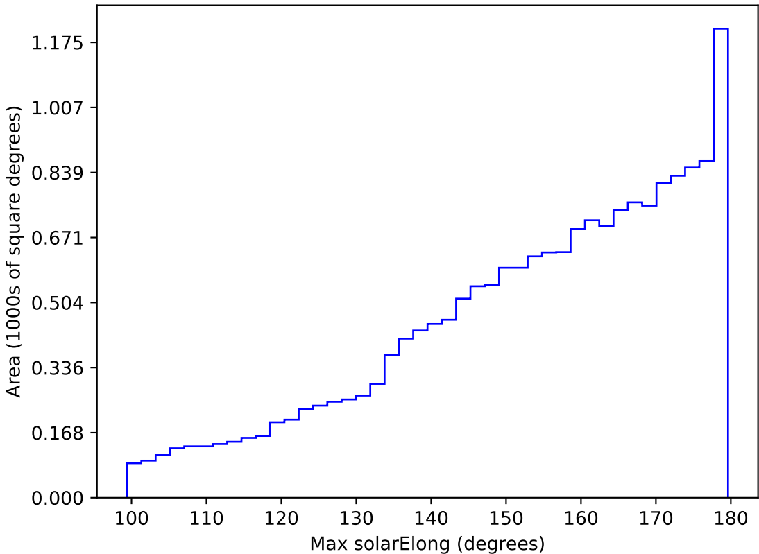
weather_cloudso12v3.4_10yrs WFD all bands: Max solarElong
