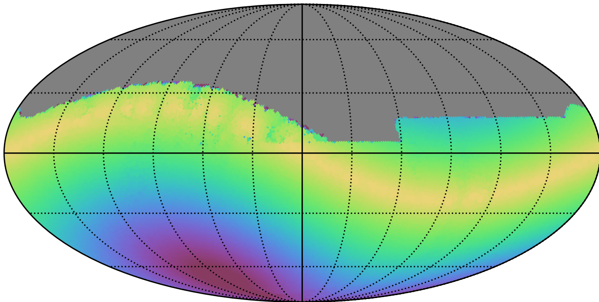
weather_cloudso12v3.4_10yrs All sky z band: Max solarElong
