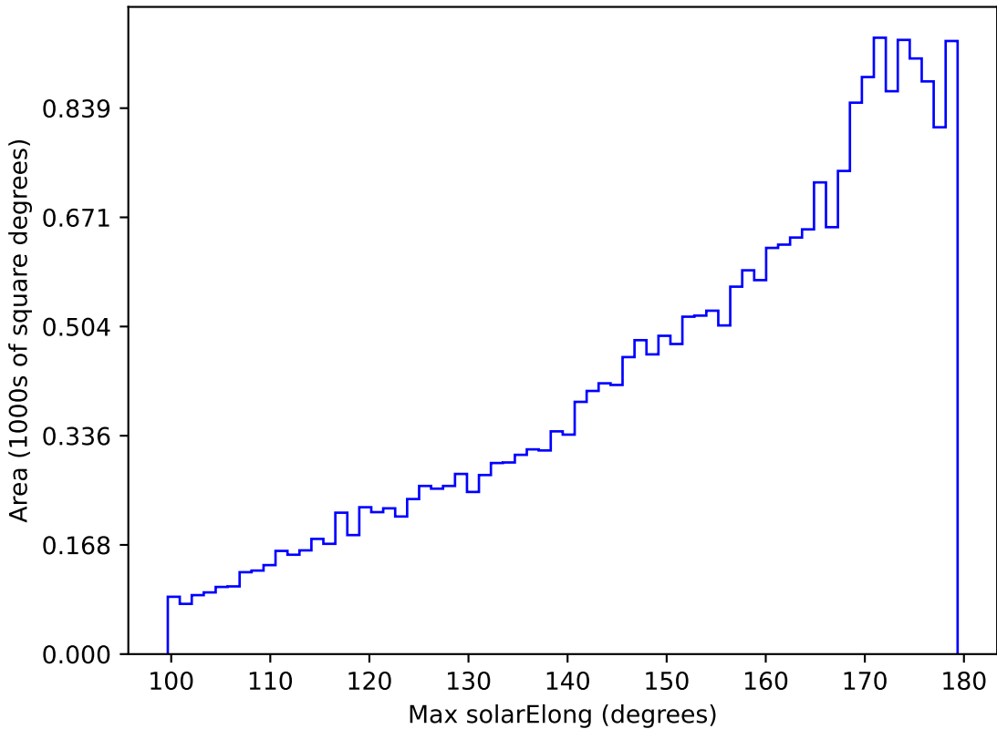
weather_cloudso12v3.4_10yrs All sky z band: Max solarElong
