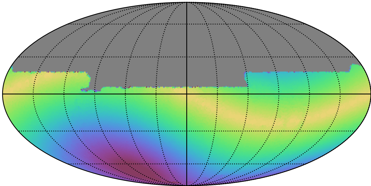
weather_cloudso12v3.4_10yrs All sky y band: Max solarElong
