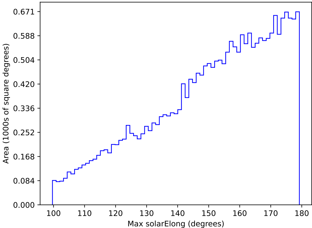
weather_cloudso12v3.4_10yrs All sky y band: Max solarElong
