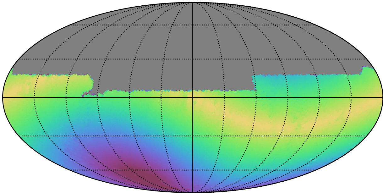
weather_cloudso12v3.4_10yrs All sky u band: Max solarElong
