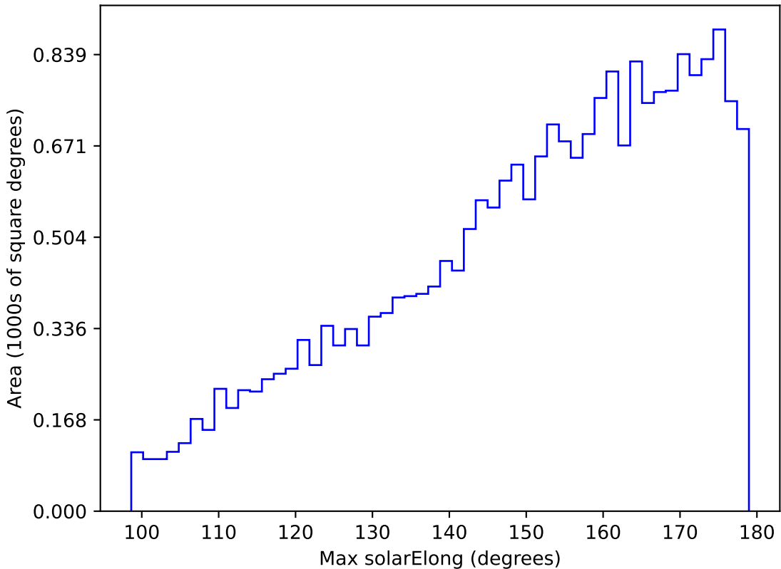
weather_cloudso12v3.4_10yrs All sky u band: Max solarElong
