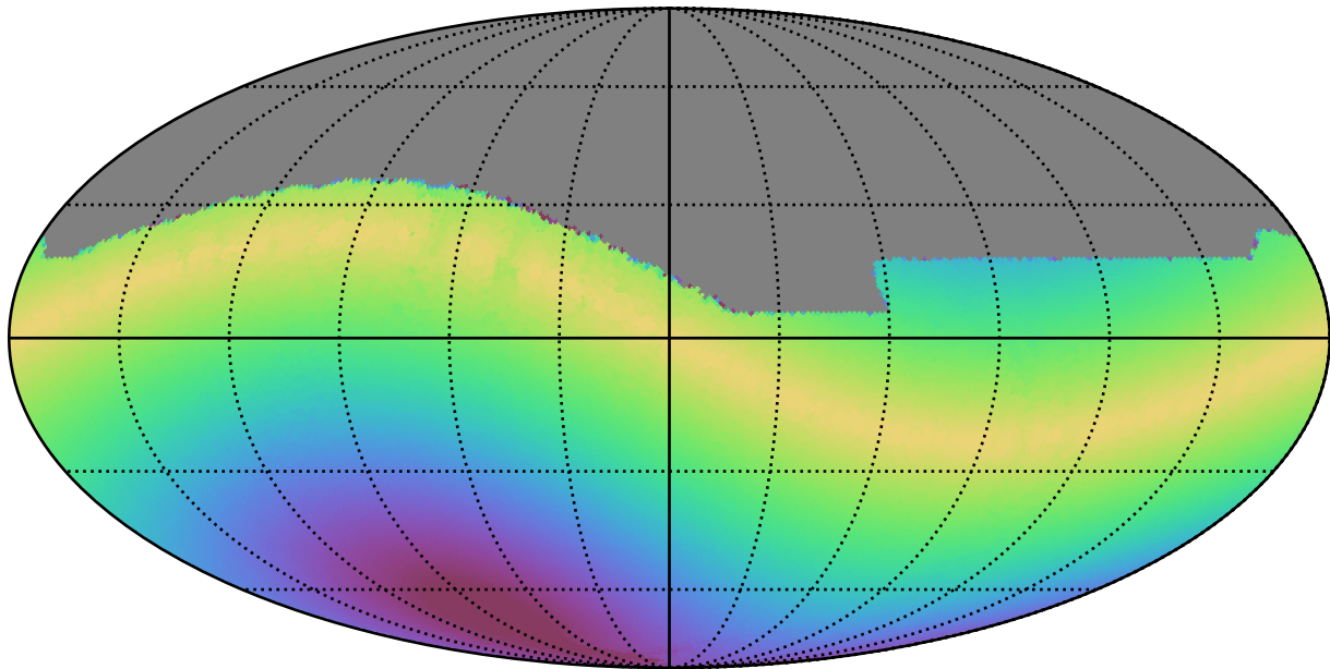
weather_cloudso12v3.4_10yrs All sky r band: Max solarElong
