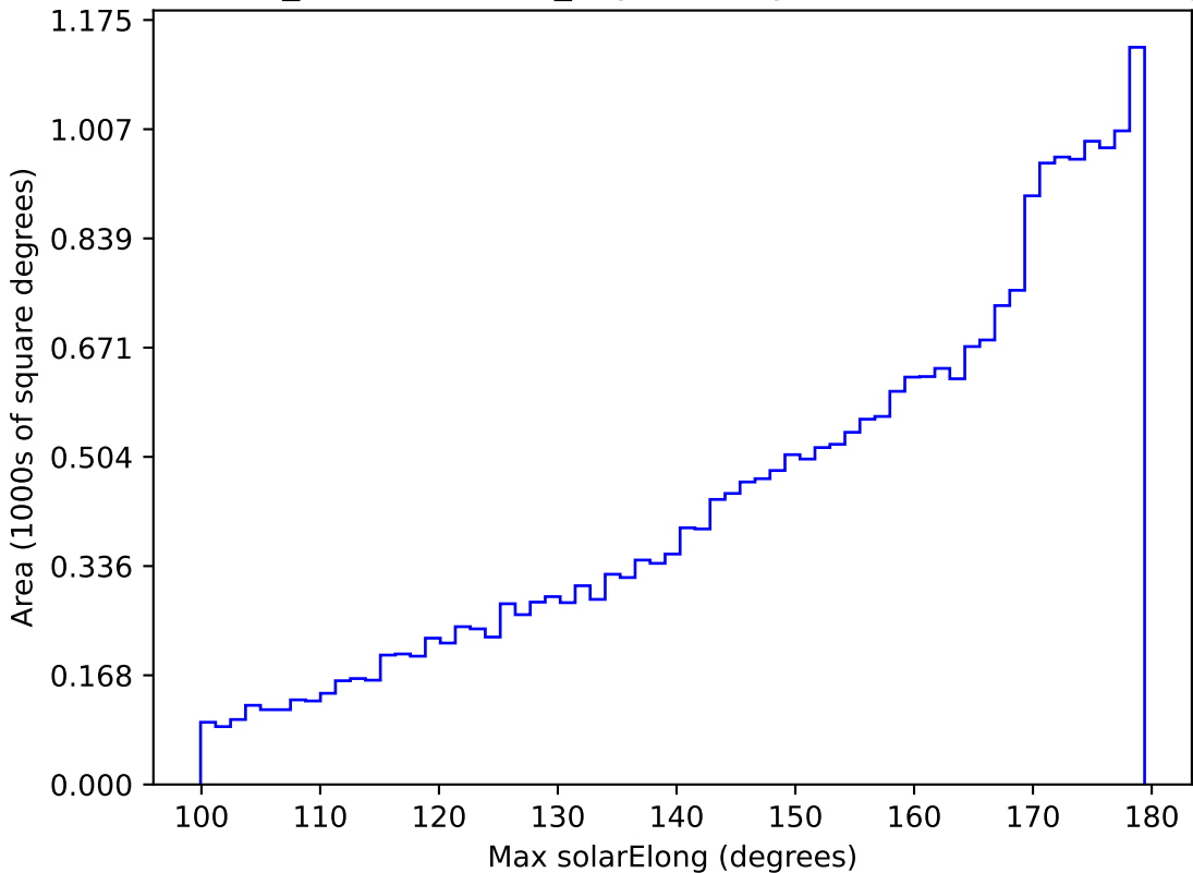
weather_cloudso12v3.4_10yrs All sky r band: Max solarElong
