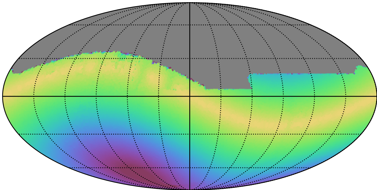
weather_cloudso12v3.4_10yrs All sky i band: Max solarElong
