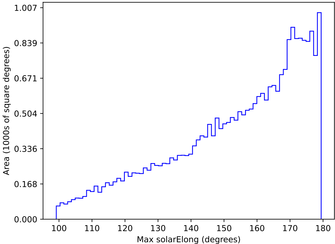
weather_cloudso12v3.4_10yrs All sky i band: Max solarElong
