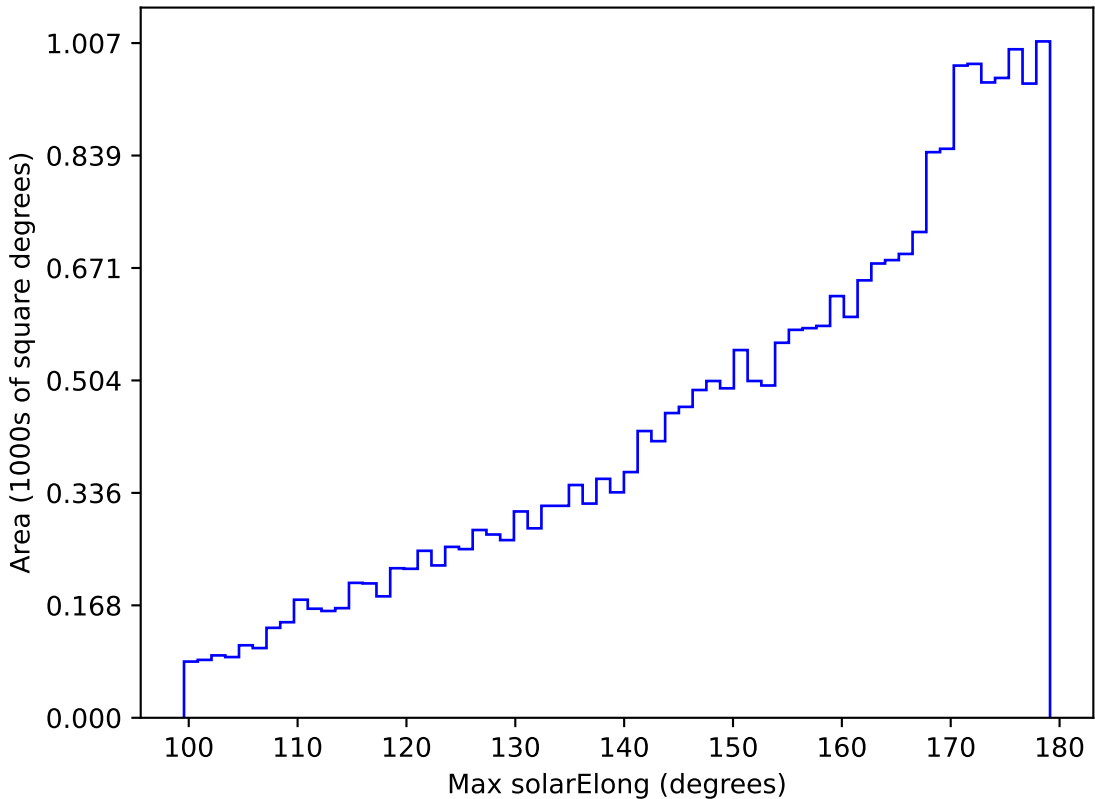
weather_cloudso12v3.4_10yrs All sky g band: Max solarElong
