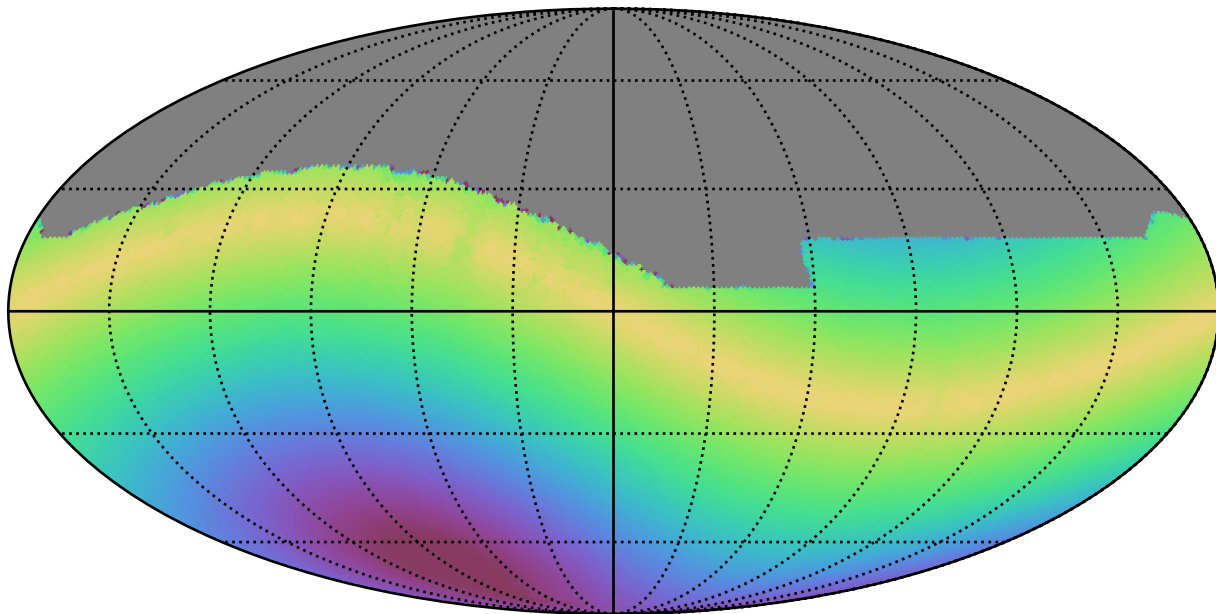
weather_cloudso12v3.4_10yrs All sky all bands: Max solarElong
