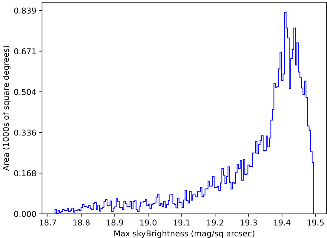
weather_cloudso12v3.4_10yrs Yr 1 z band: Max skyBrightness
