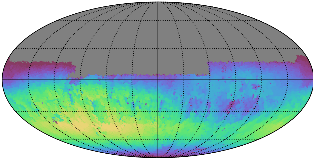
weather_cloudso12v3.4_10yrs Yr 1 u band: Max skyBrightness
