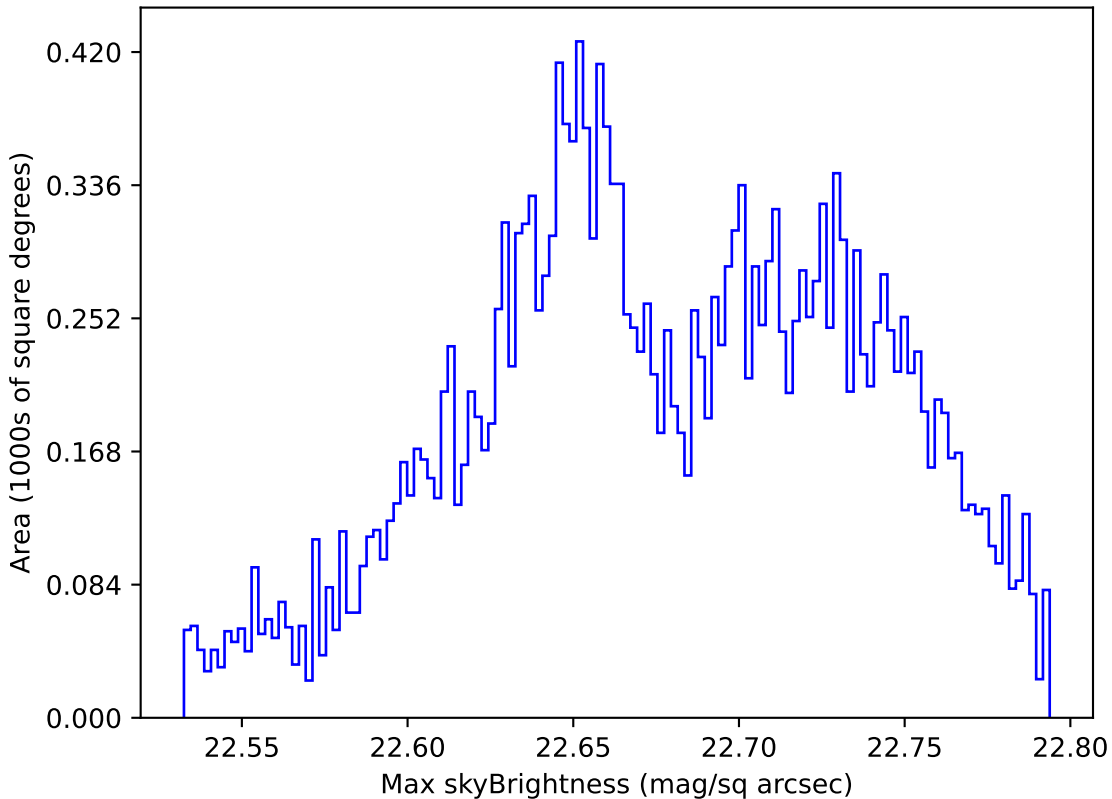
weather_cloudso12v3.4_10yrs Yr 1 u band: Max skyBrightness
