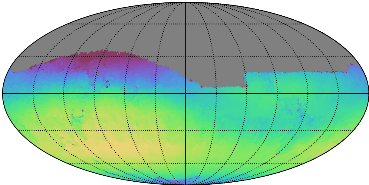
weather_cloudso12v3.4_10yrs Yr 1 r band: Max skyBrightness
