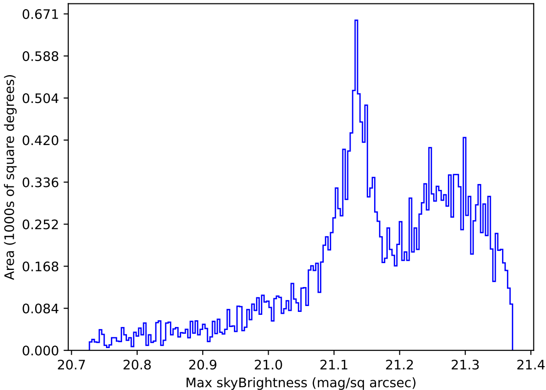
weather_cloudso12v3.4_10yrs Yr 1 r band: Max skyBrightness
