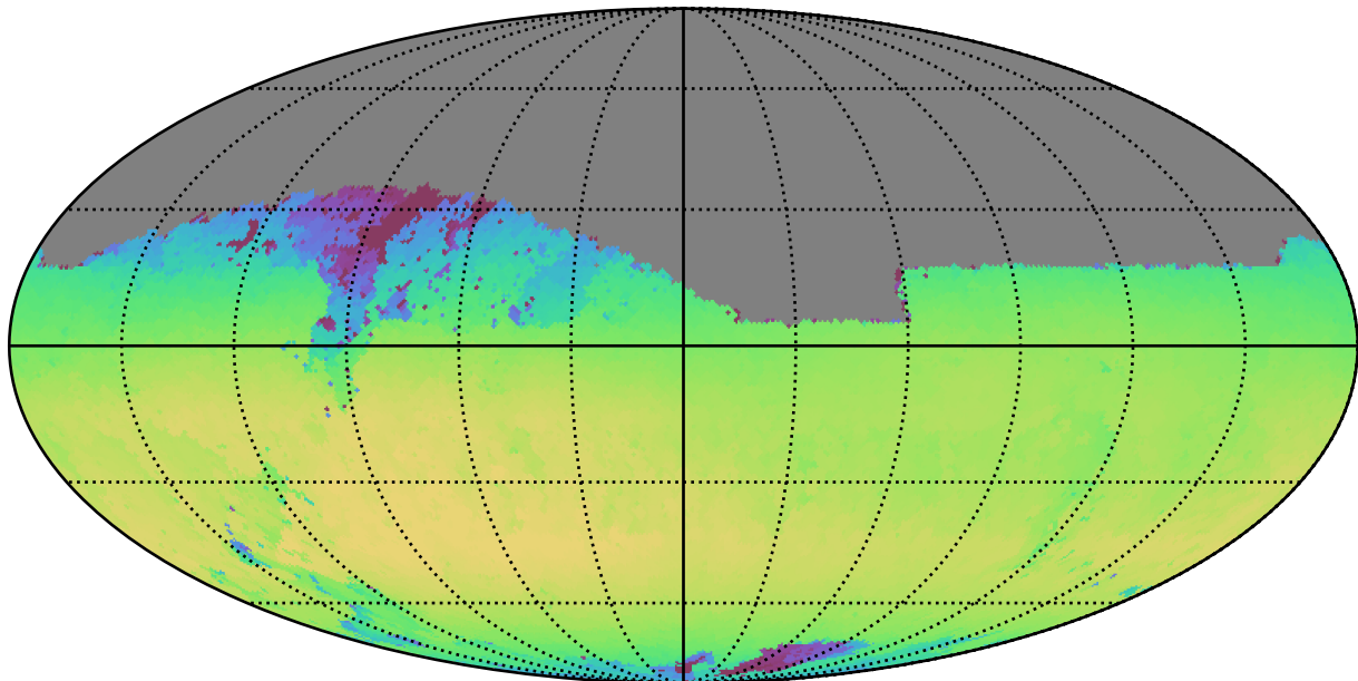
weather_cloudso12v3.4_10yrs Yr 1 i band: Max skyBrightness
