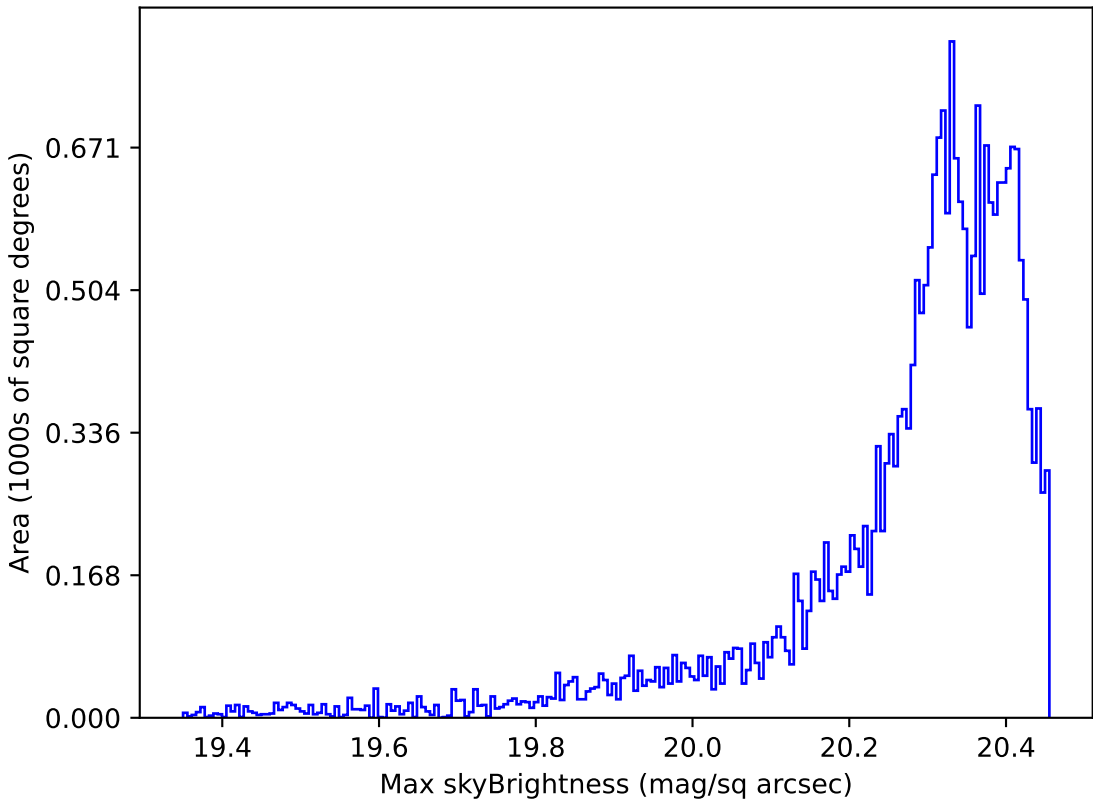
weather_cloudso12v3.4_10yrs Yr 1 i band: Max skyBrightness
