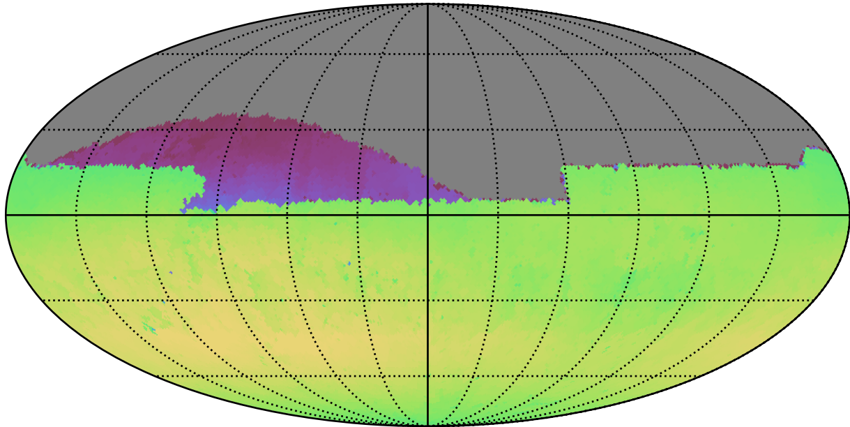
weather_cloudso12v3.4_10yrs Yr 1 all bands: Max skyBrightness
