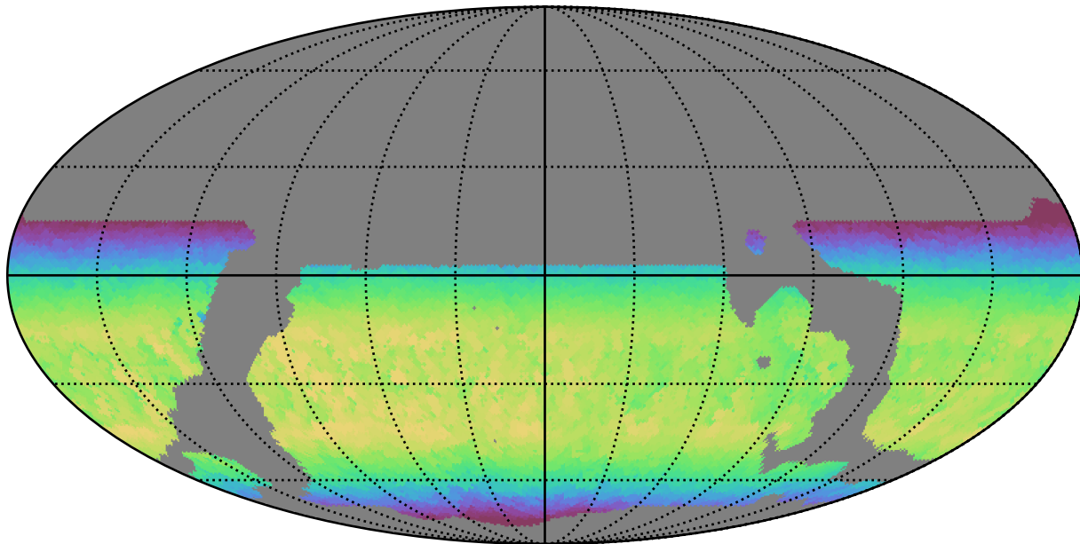
weather_cloudso12v3.4_10yrs WFD y band: Max skyBrightness
