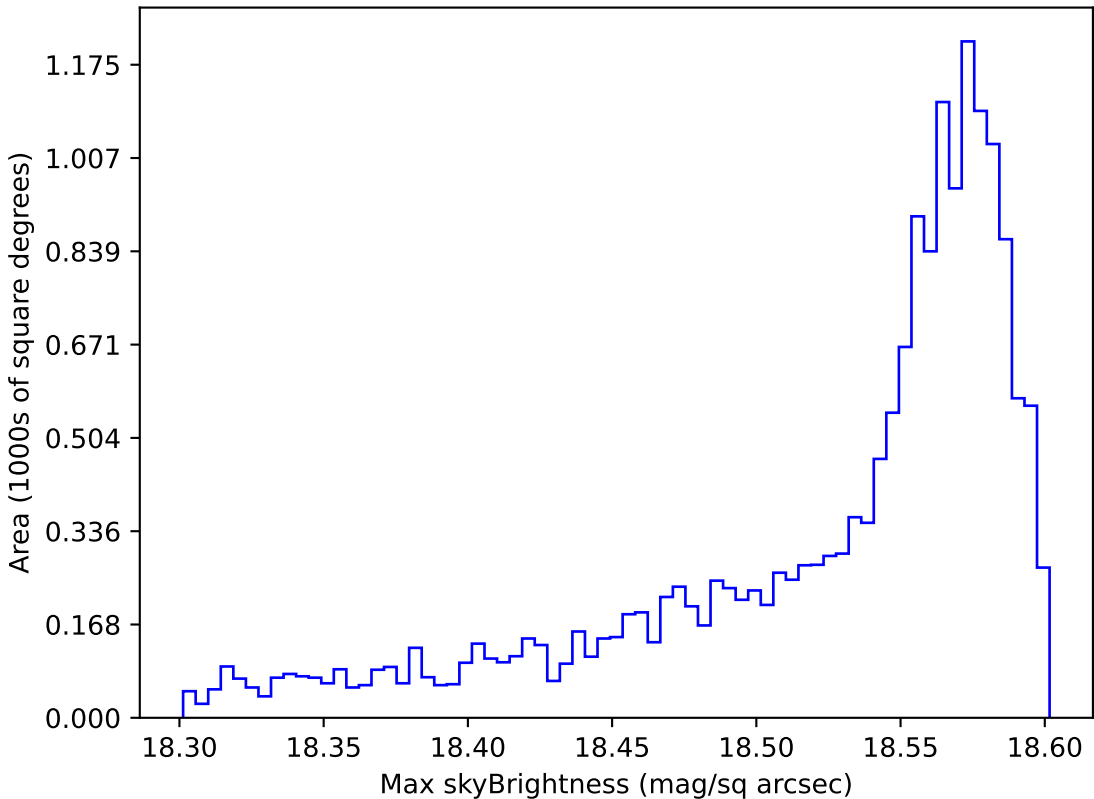
weather_cloudso12v3.4_10yrs WFD y band: Max skyBrightness
